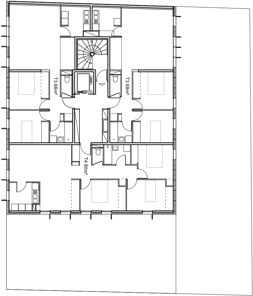
PLAN R+3
