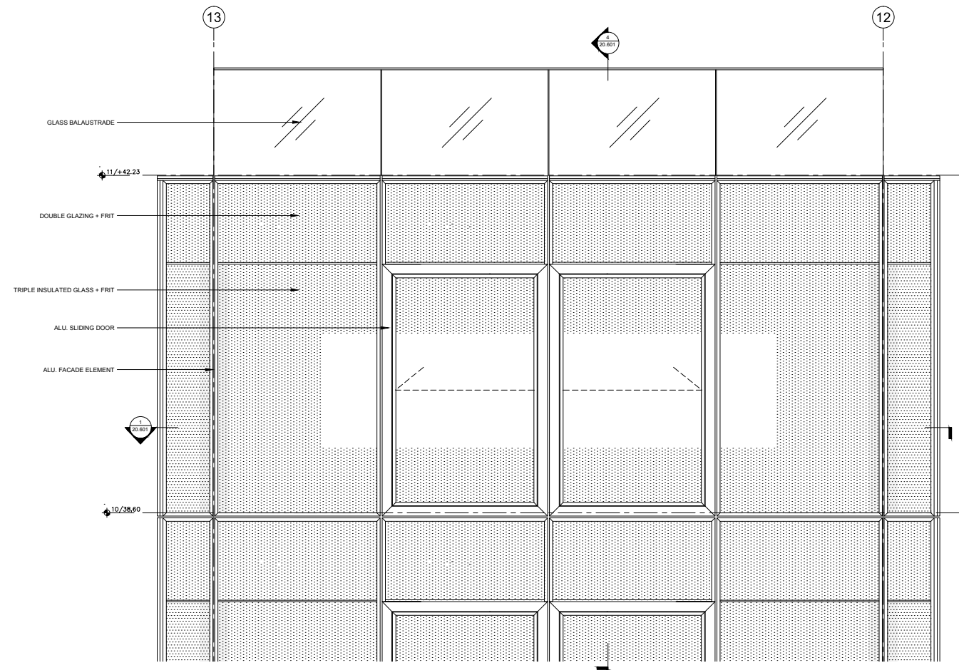
2 PARTIAL ELEVATION SCALE 1:20
