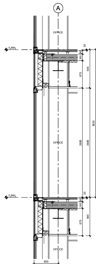
3 PARTIAL SECTION SCALE 1:20
