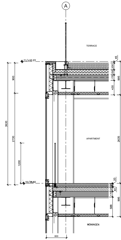
4 PARTIAL SECTION SCALE 1:20
