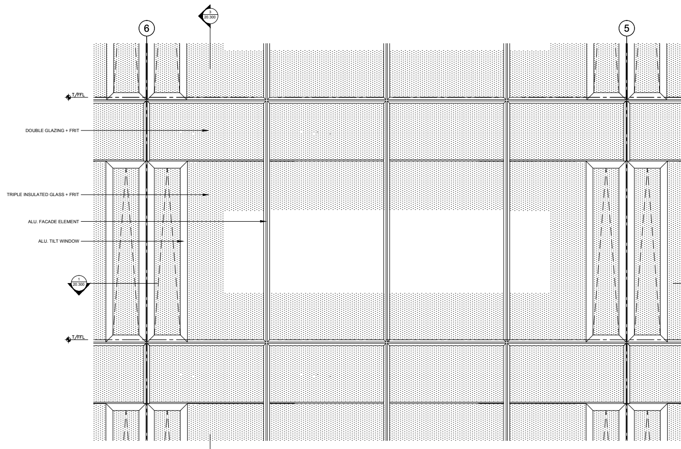
2 PARTIAL ELEVATION SCALE 1:20
