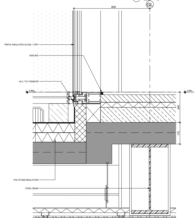
6 VERTICAL DETAIL SCALE 1:5
