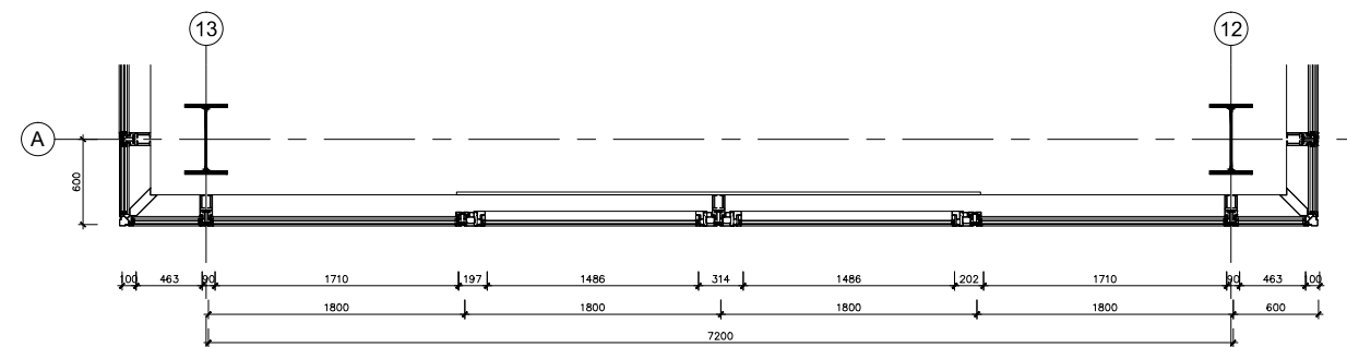
1 PARTIAL PLAN SCALE 1:20
