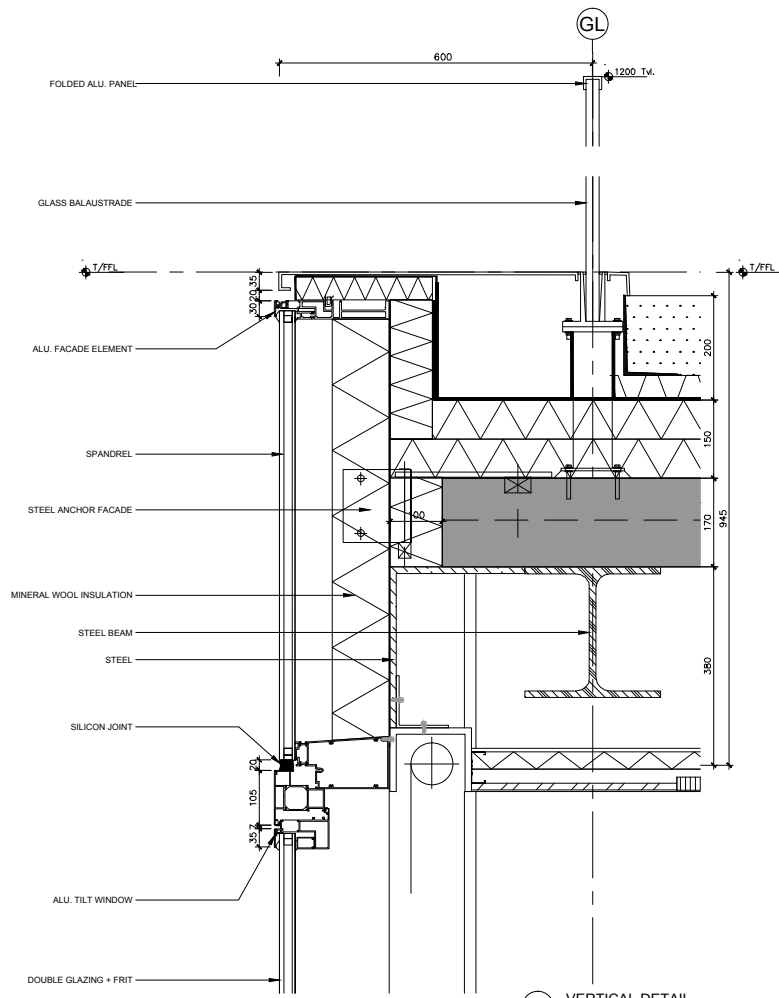
6 VERTICAL DETAIL SCALE 1:5
