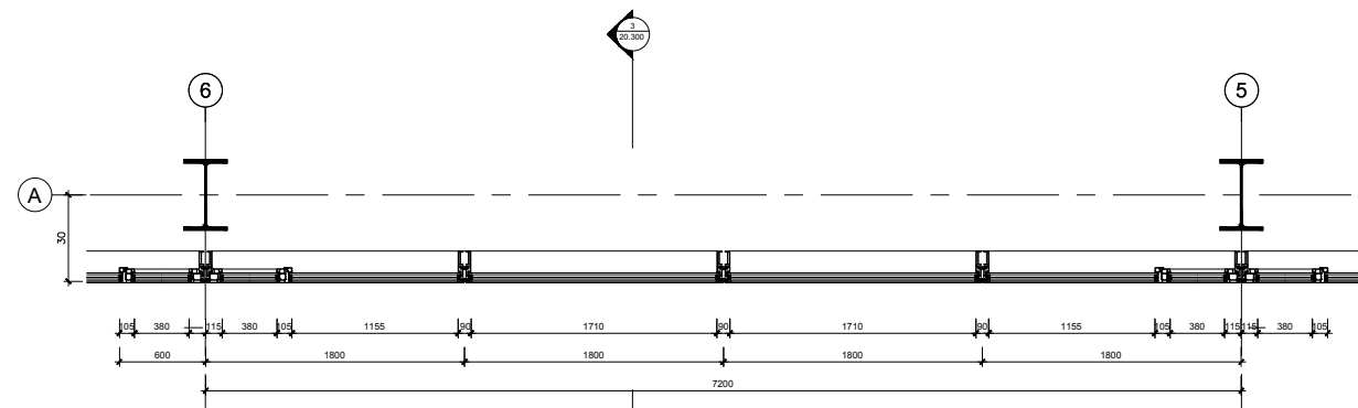
1 PARTIAL PLAN SCALE 1:20
